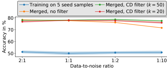
Figure 3: Performance development with different data-to-noise ratios. Here, baseline refers to training with 5 random positive samples from the CUB200-2011 training images. The merged dataset is this seed dataset joined with the different augment datasets of different data-to-noise ratios. Our filter method was tested with two different values for k . Then, the filtered datasets together with the seed dataset were used to train a classification model.
