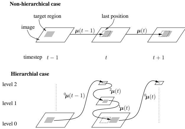
Figure 1. Propagation of the estimated motion parameter vector \mu over time. In the non-hierarchical case (top) only small image motions can be tracked properly. In the hierarchical case (bottom) larger motions can be handled. Here, it is depicted for a hierarchy with three levels.
