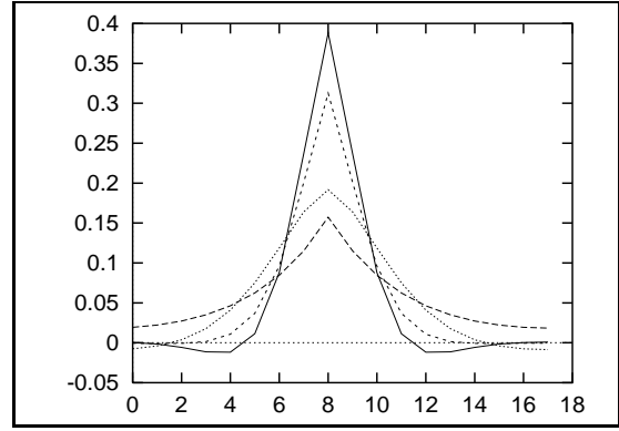
Figure 1: Influence of the snake elements on the position of the 8th element for different combinations of \alpha and \beta using a constant matrix \mathbf{A} ( x -axis: snake element, y -axis: influence of the snake element’s position).
