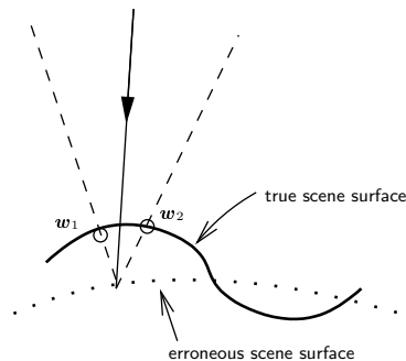
Figure 2: Interpolation with depth uncertainty. A viewing ray (solid line) is interpolated from two recorded viewing rays (dashed lines) that have been selected assuming an erroneous scene surface.
