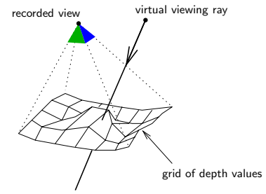
Figure 3: Intersection of the viewing ray with the depth map as search between the planes of minimum and maximum depth.
